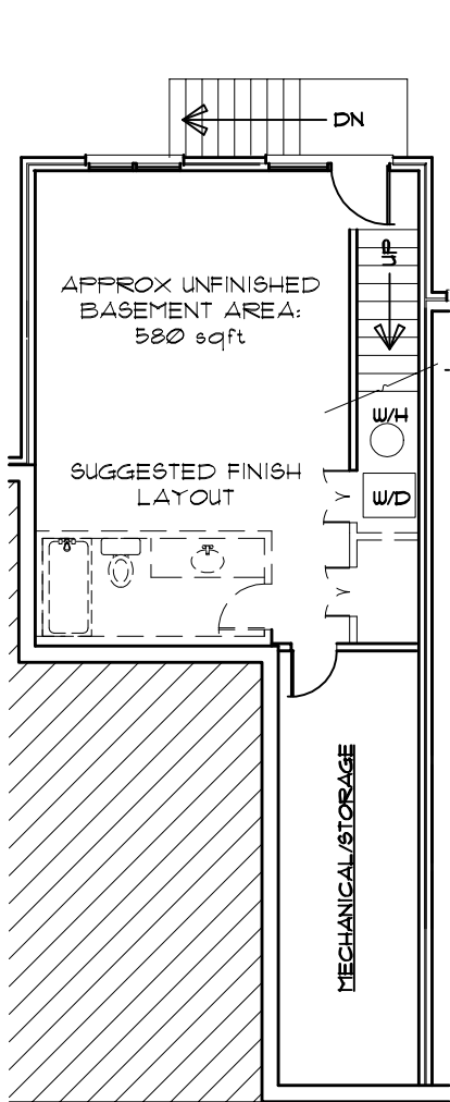
BASEMENT PLAN
