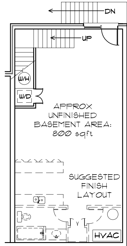
BASEMENT PLAN
